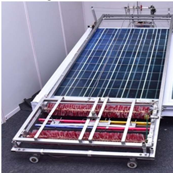
Net Zero Automatic Solar Panel Cleaning Robot
