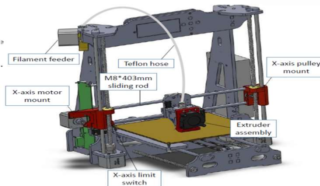
3d Printer
