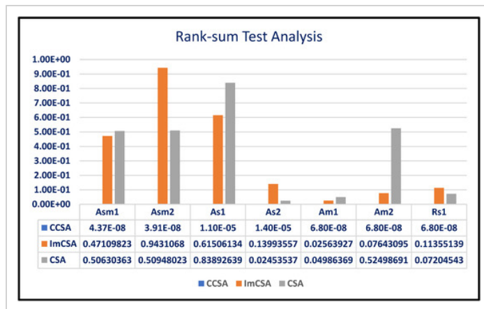
Figure 6. Rank-sum Test Analysis.
