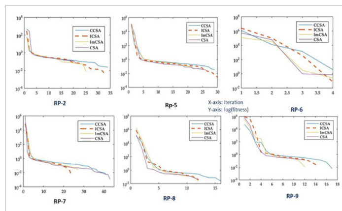
Figure 7. Convergence property analysis.
