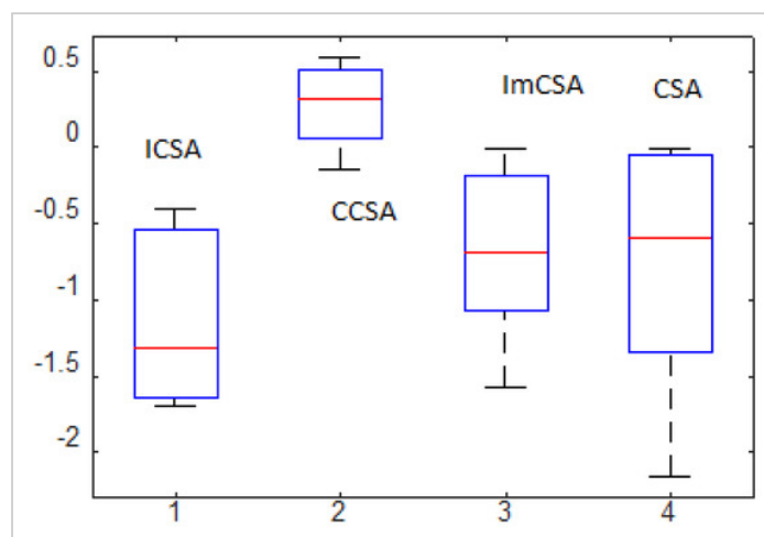
Figure 4. BPA for Am1.
