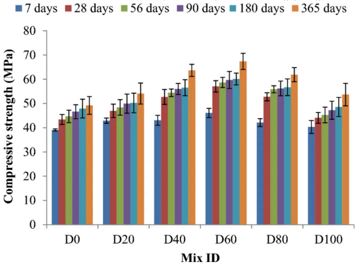
Influence of CWTA on compressive strength of SCC
