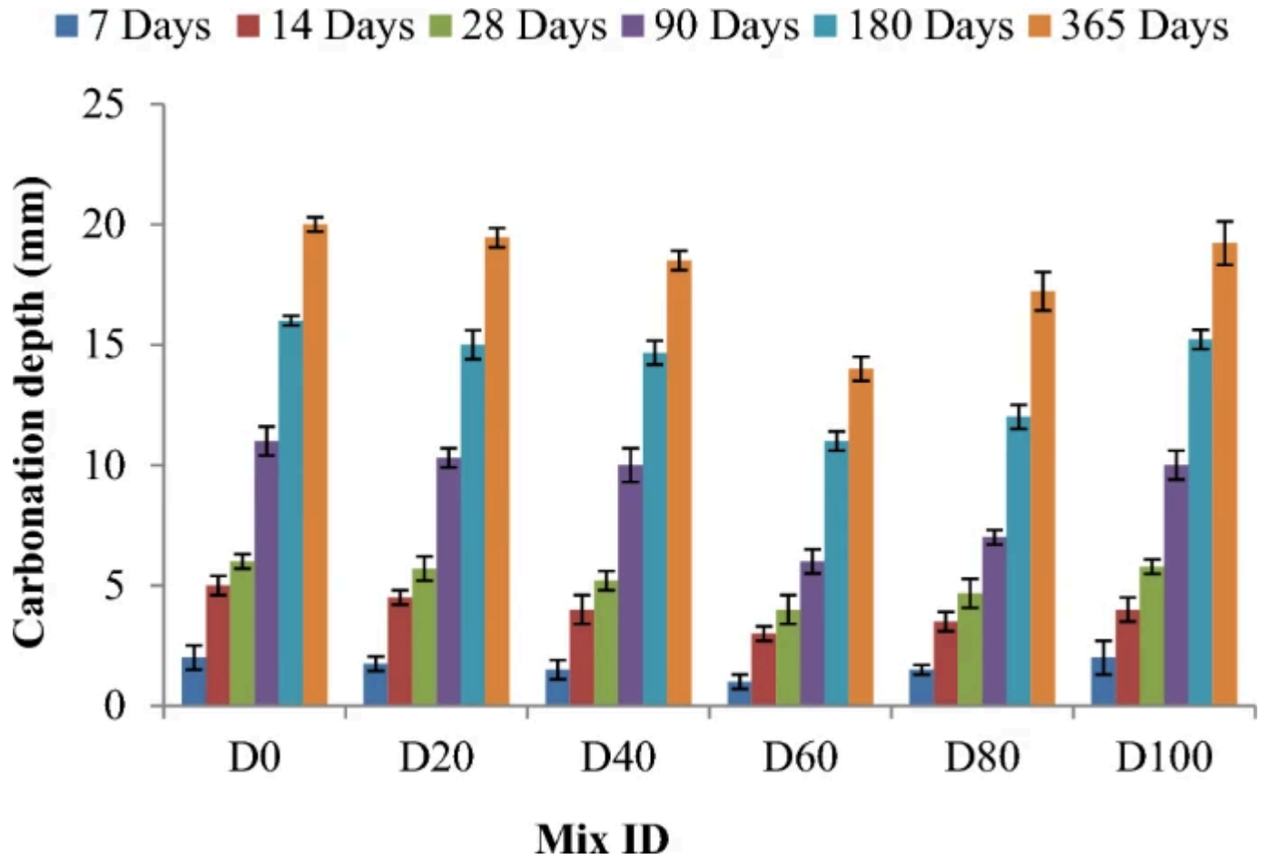
Influence of CWTA on carbonation depth of SCC mixtures
