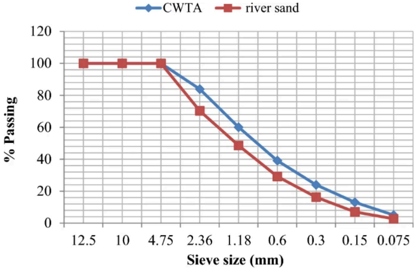
Gradation of river sand and CWTA
