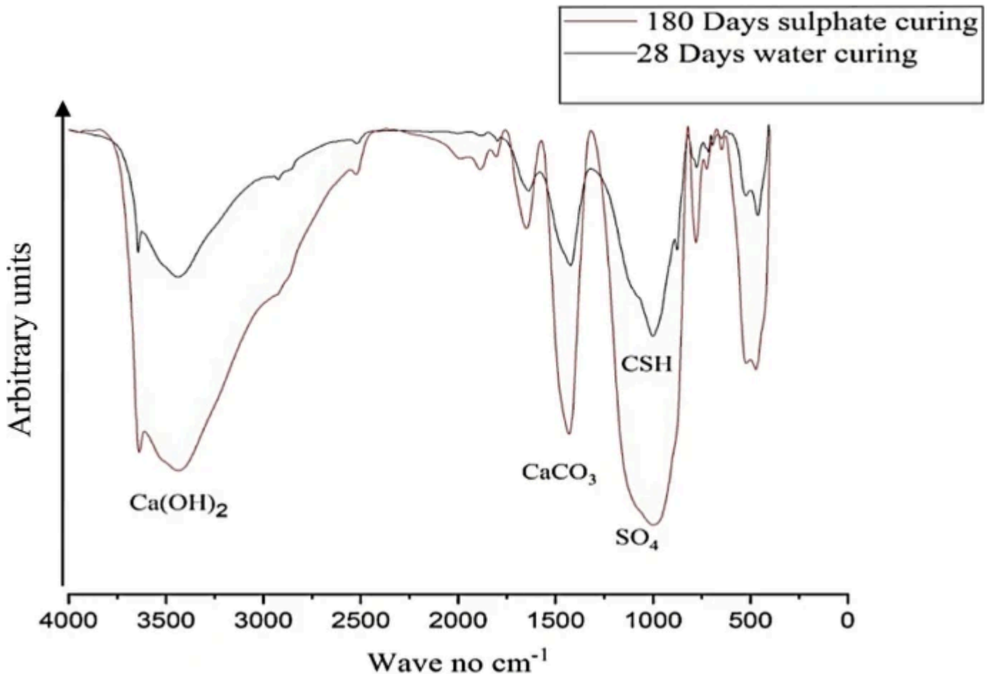
FTIR spectra for D 20 mix at 180 days MgSO 4 exposure period
