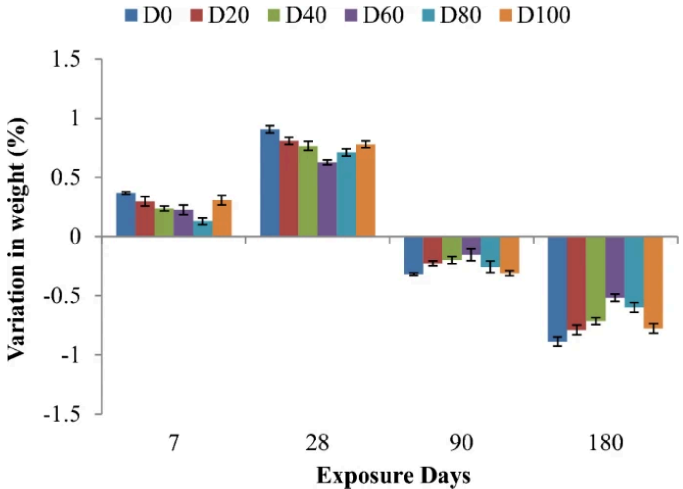
Variation in weight of CWTA-based SCC after exposure to sulphate attack
