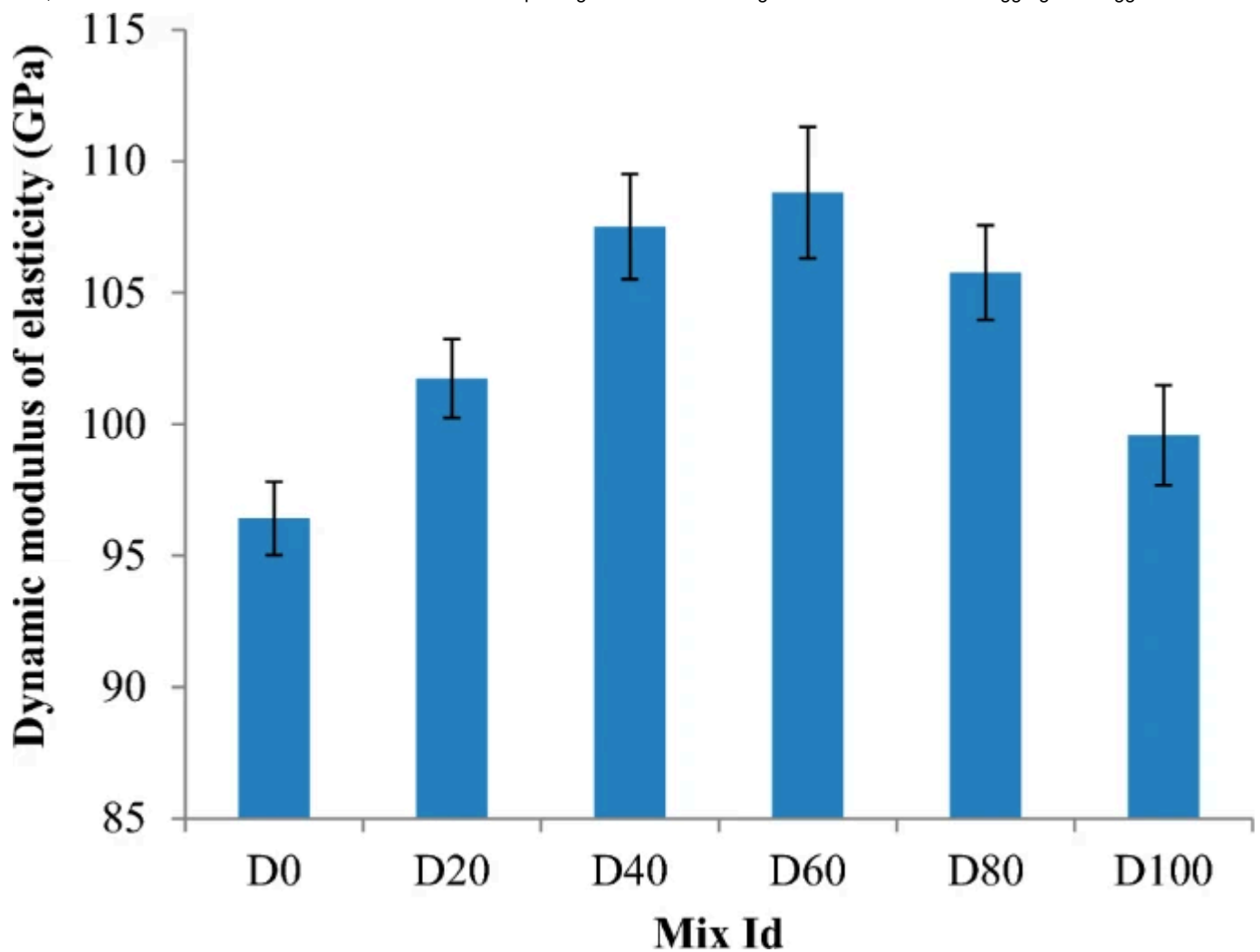
Influence of CWTA on DME of SCC mixtures
