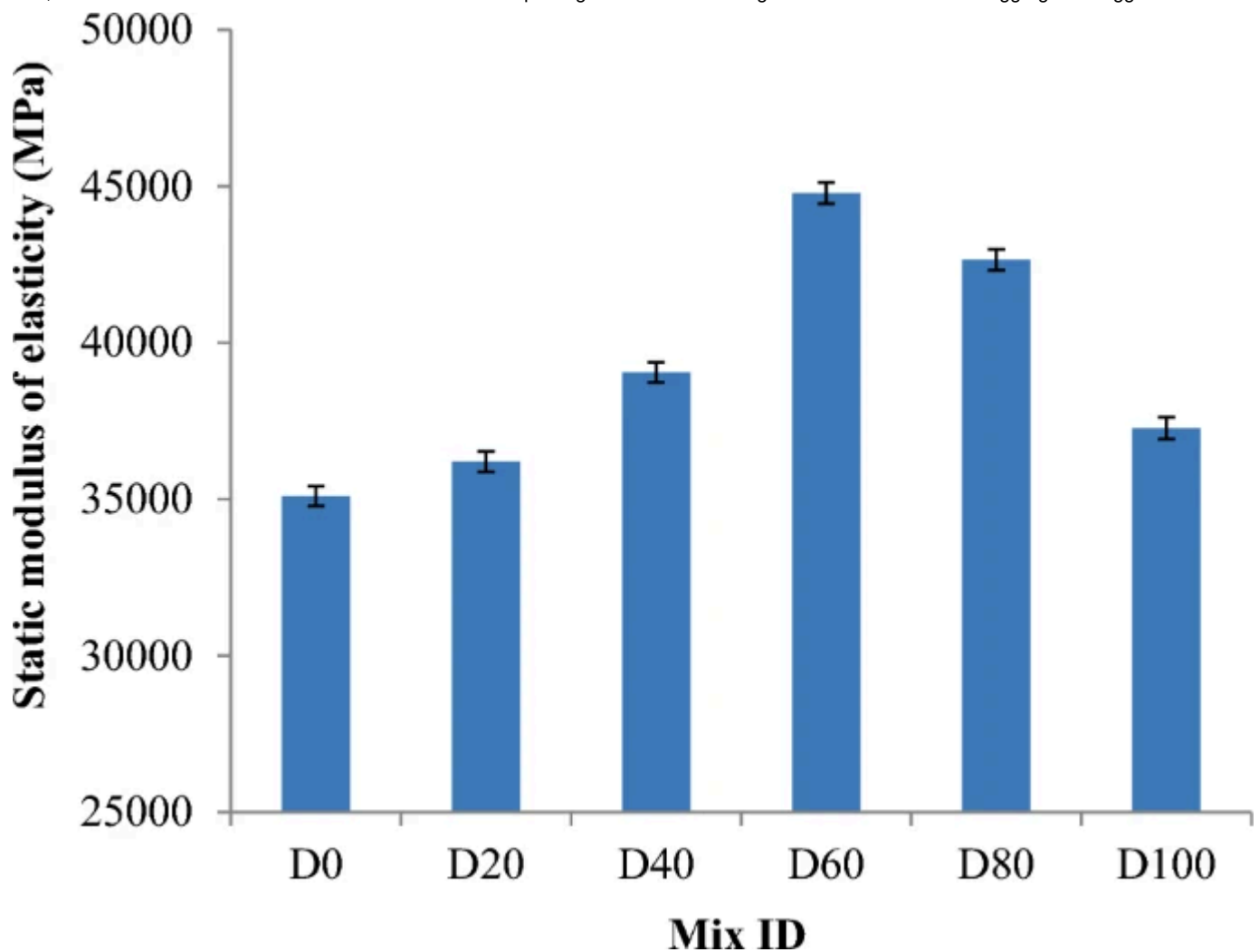
Influence of CWTA on SME of SCC
