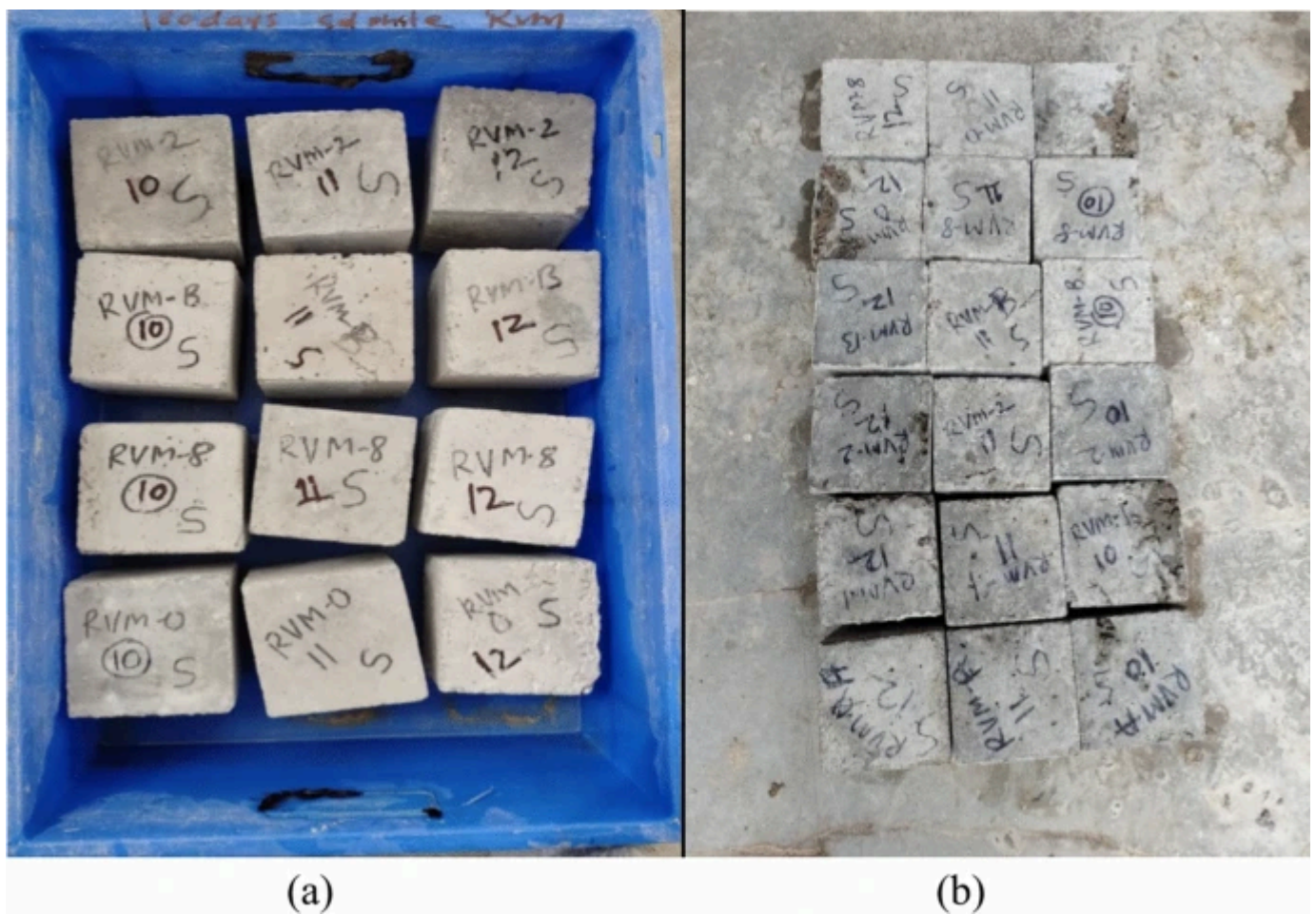
SCC specimens exposed to \text{MgSO}_4 solution a 0 days b 180 days
