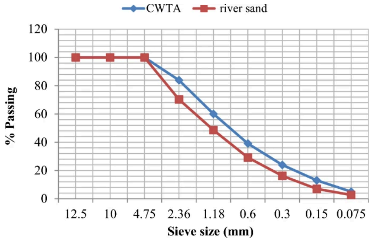
Gradation of river sand and CWTA
