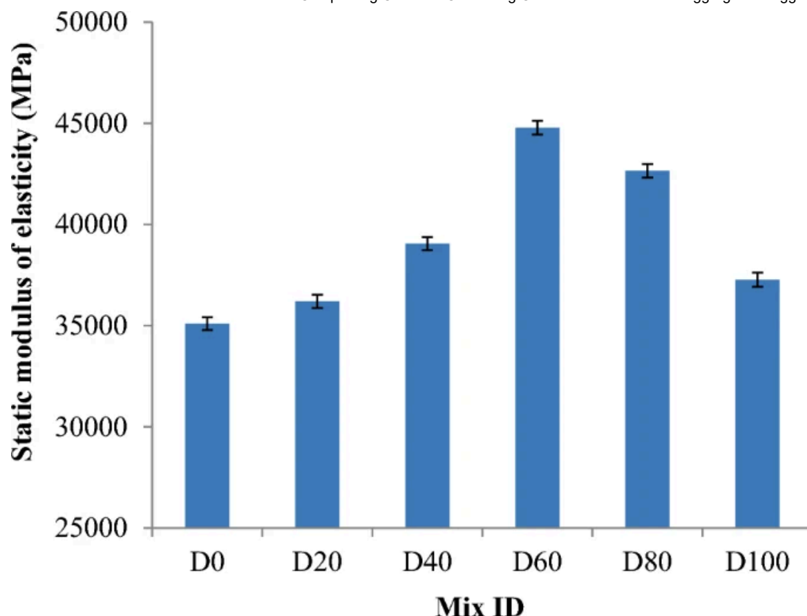
Influence of CWTA on SME of SCC
