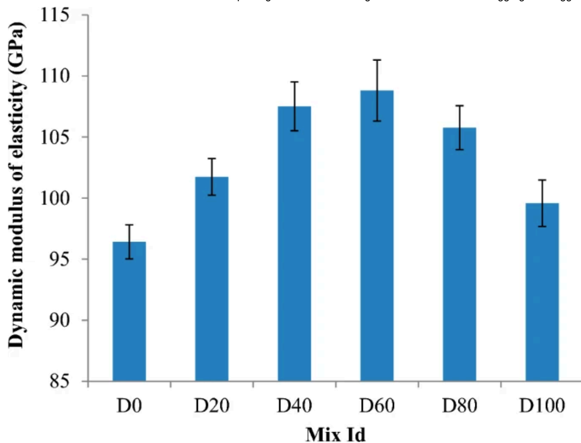
Influence of CWTA on DME of SCC mixtures
