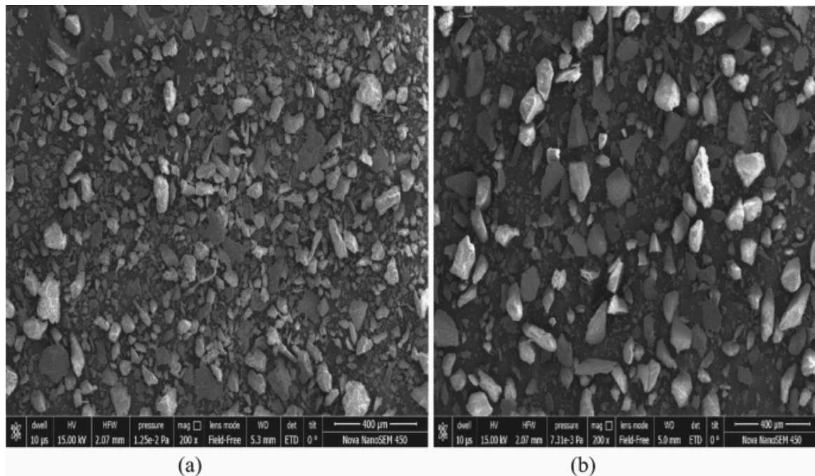
SEM images a CWTA b River sand
