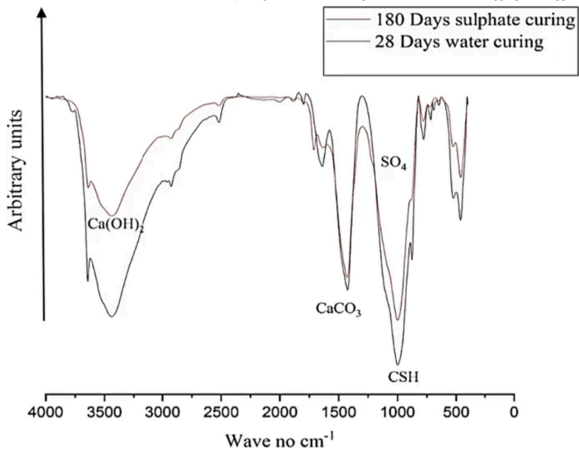
FTIR spectra for D 0 mix at 180 days MgSO 4 exposure period
