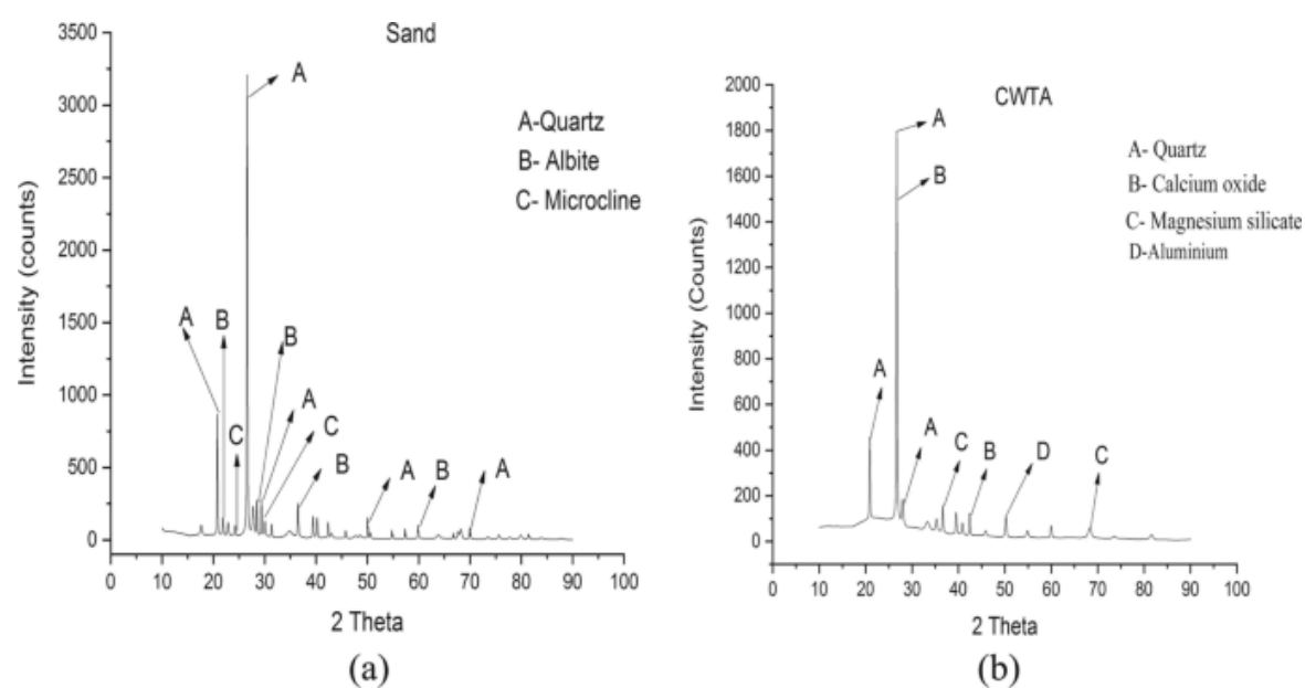
XRD patterns a River sand b CWTA
