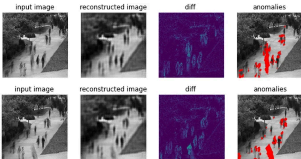
Predictions from the LSTM autoencoder model
