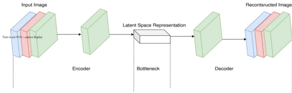
Architecture of convolutional autoencoder
