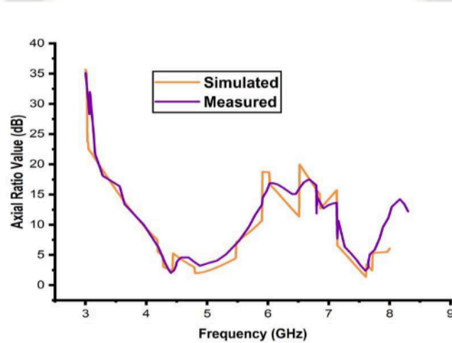
Figure 9: Comparison between simulated and measured axial ratio variations of design 4 with frequency
