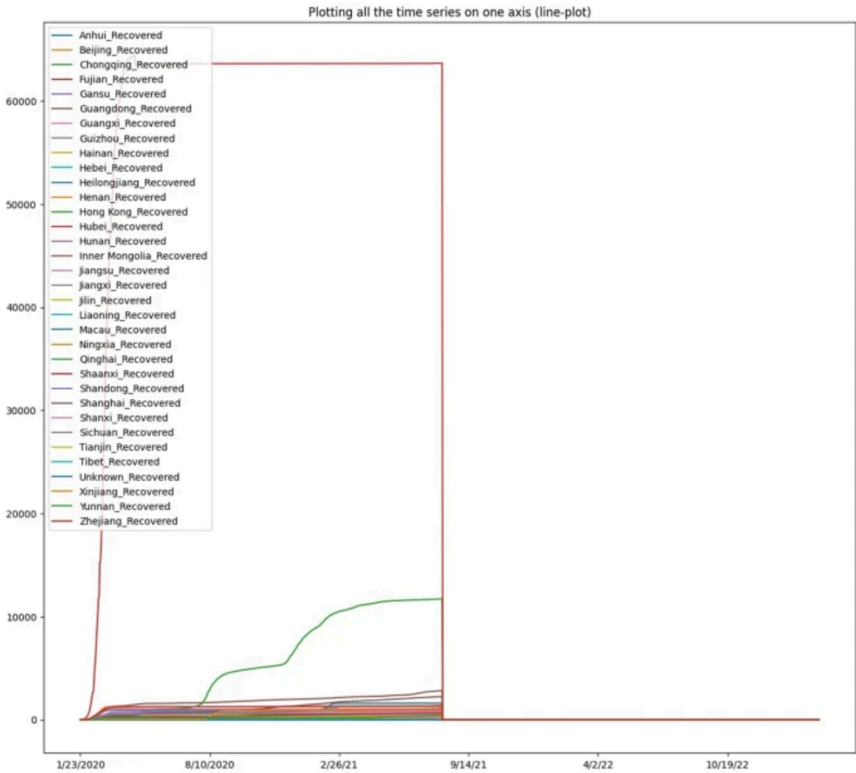
TSP of recovered cases in China
