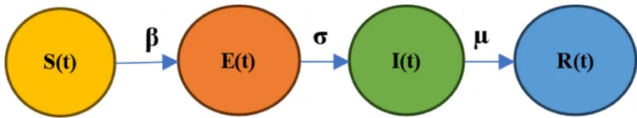
SEIR epidemiological model
