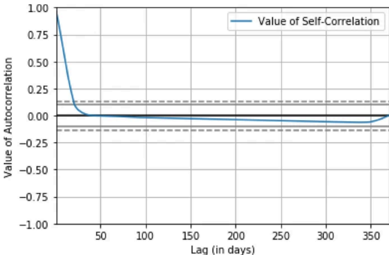
Autocorrelation plot for confirmed cases in Hubei
