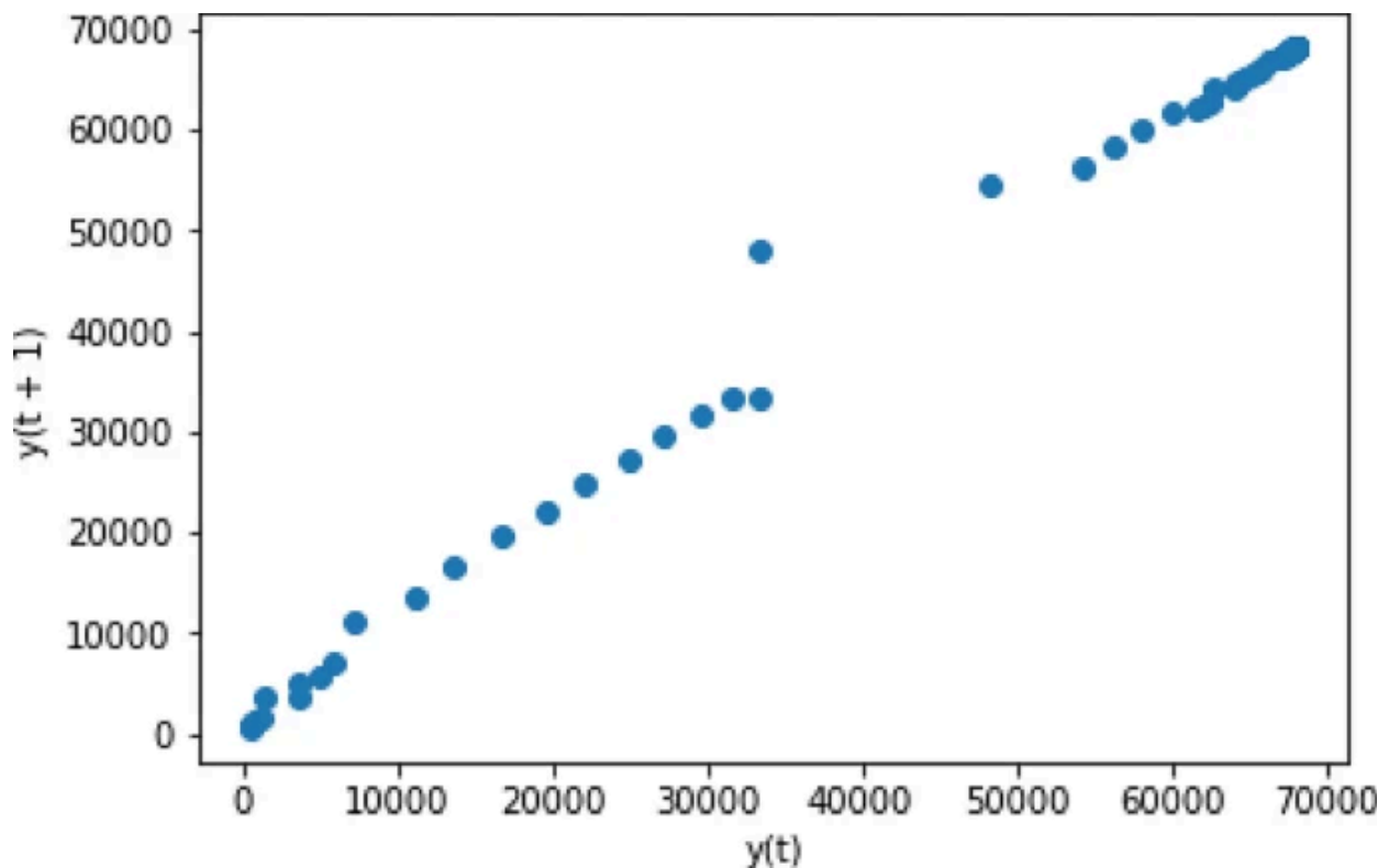
Scatter plot of confirmed cases in Hubei
