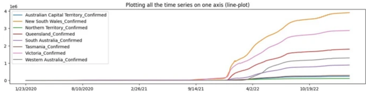
Confirmed cases in Australia
