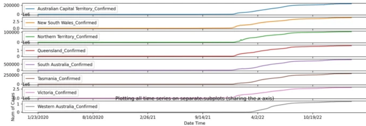
Statewide confirmed cases in Australia
