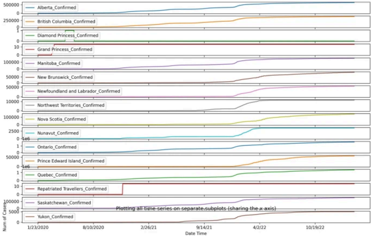
Statewide confirmed cases in Canada
