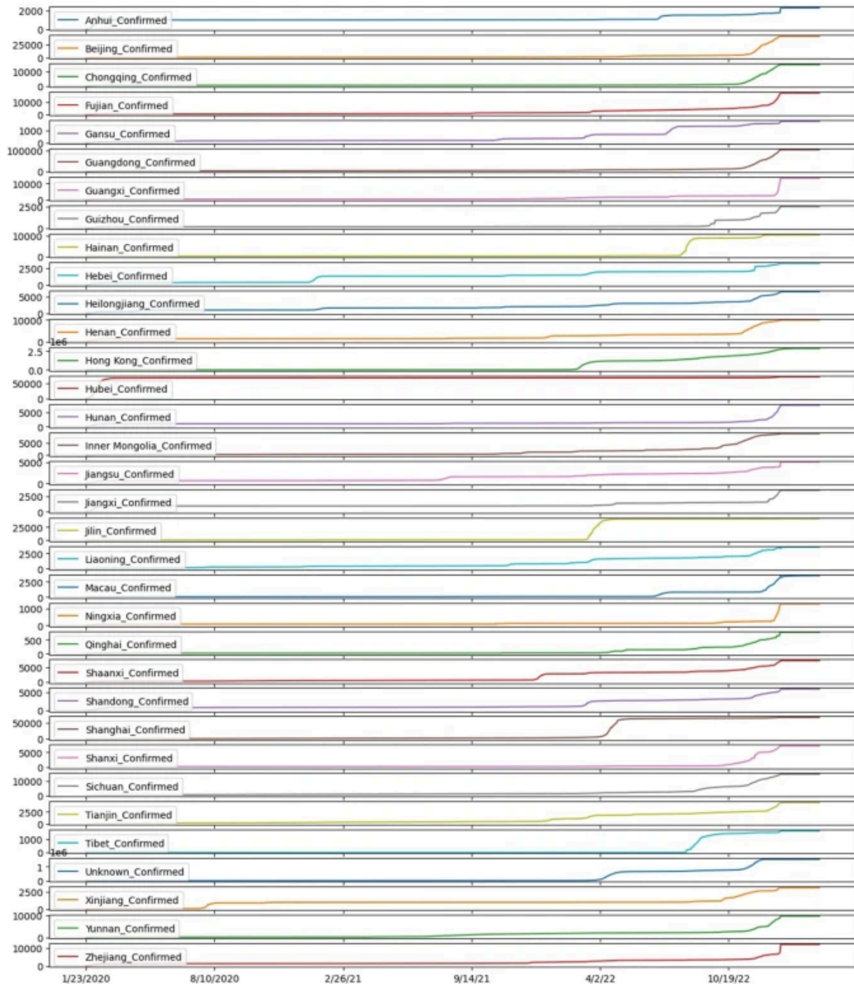
TSP of province-wide confirmed cases in China
