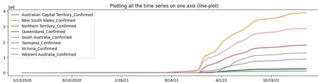
Confirmed cases in Australia
