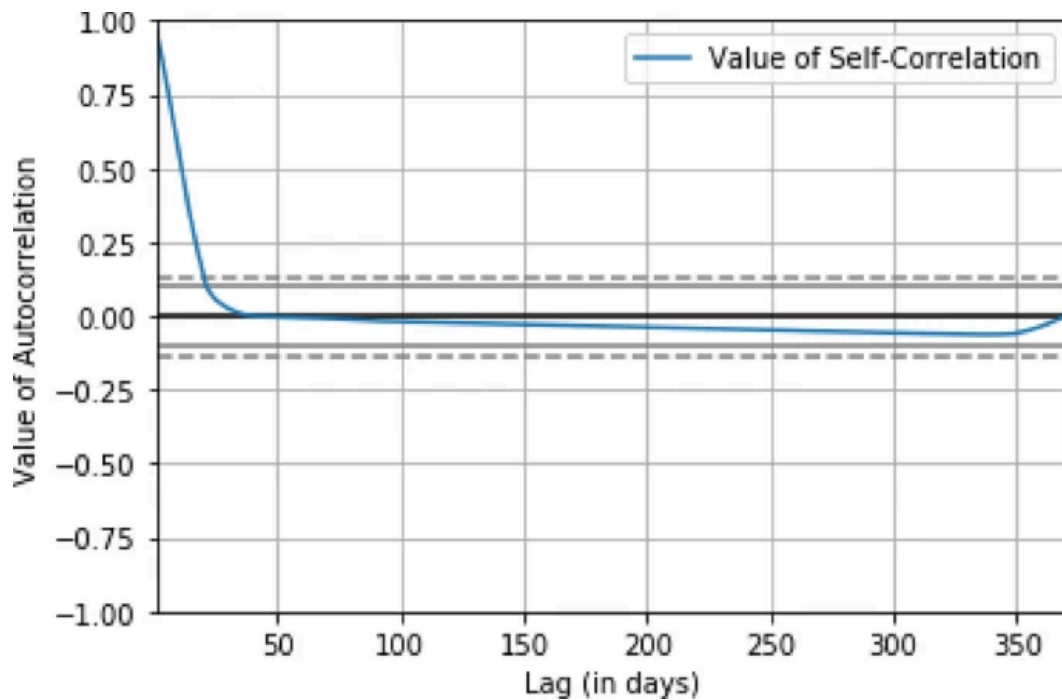
Autocorrelation plot for confirmed cases in Hubei
