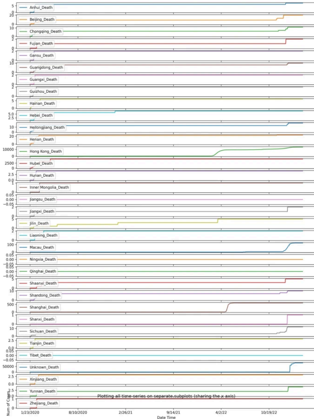
TSP for death cases in China according to each province
