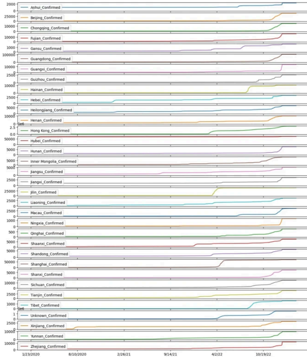
TSP of province-wide confirmed cases in China
