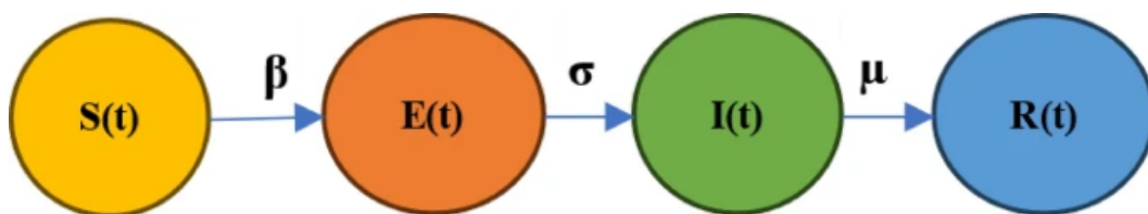
SEIR epidemiological model
