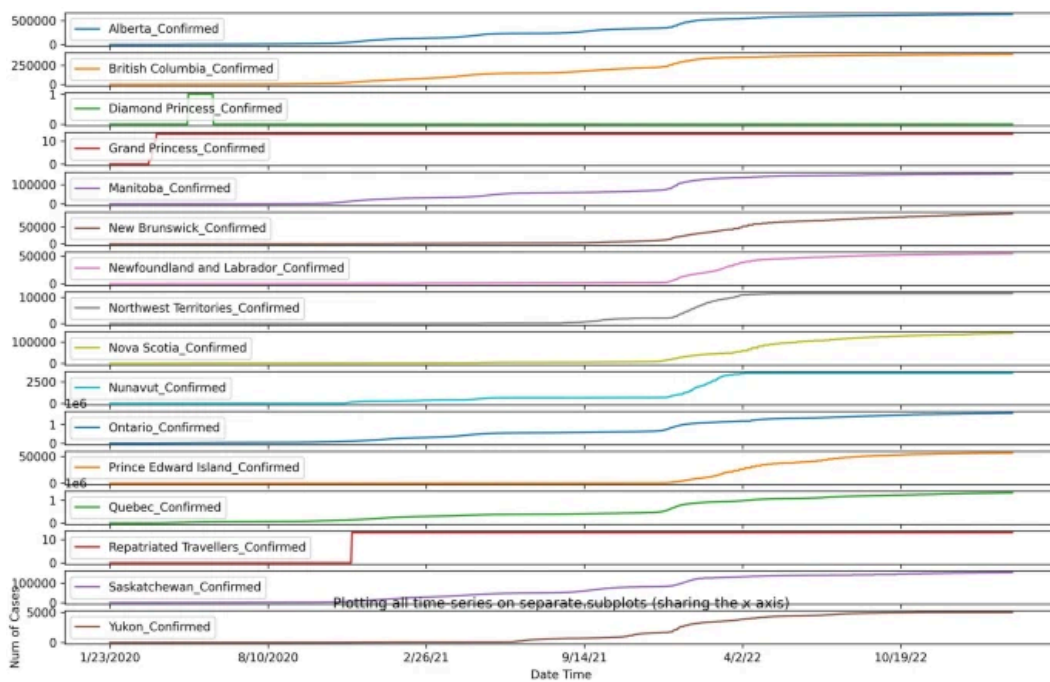
Statewide confirmed cases in Canada
