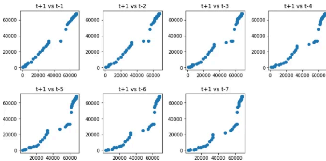
Scatter plot for different time limits
