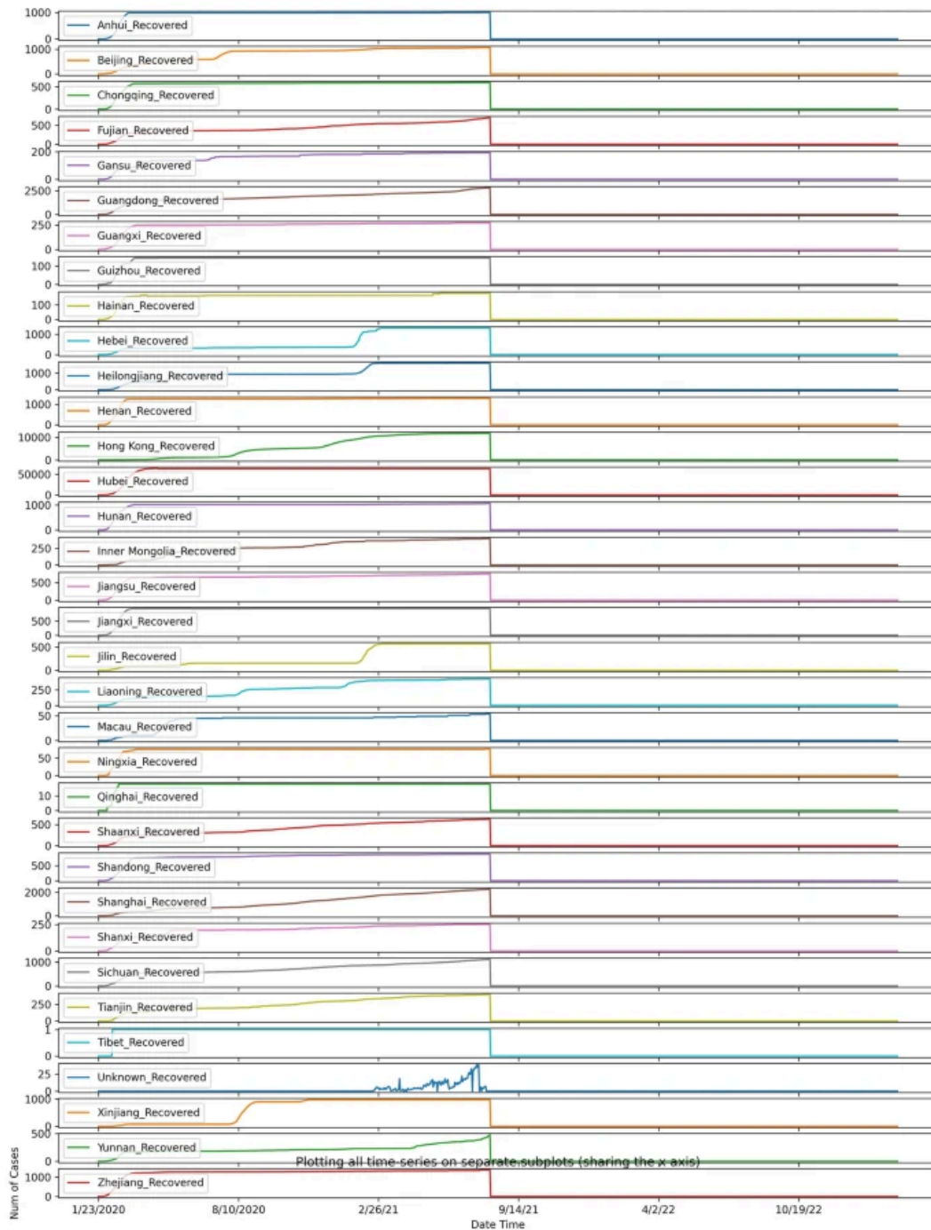
Province-wide TSP for recovered cases in China
