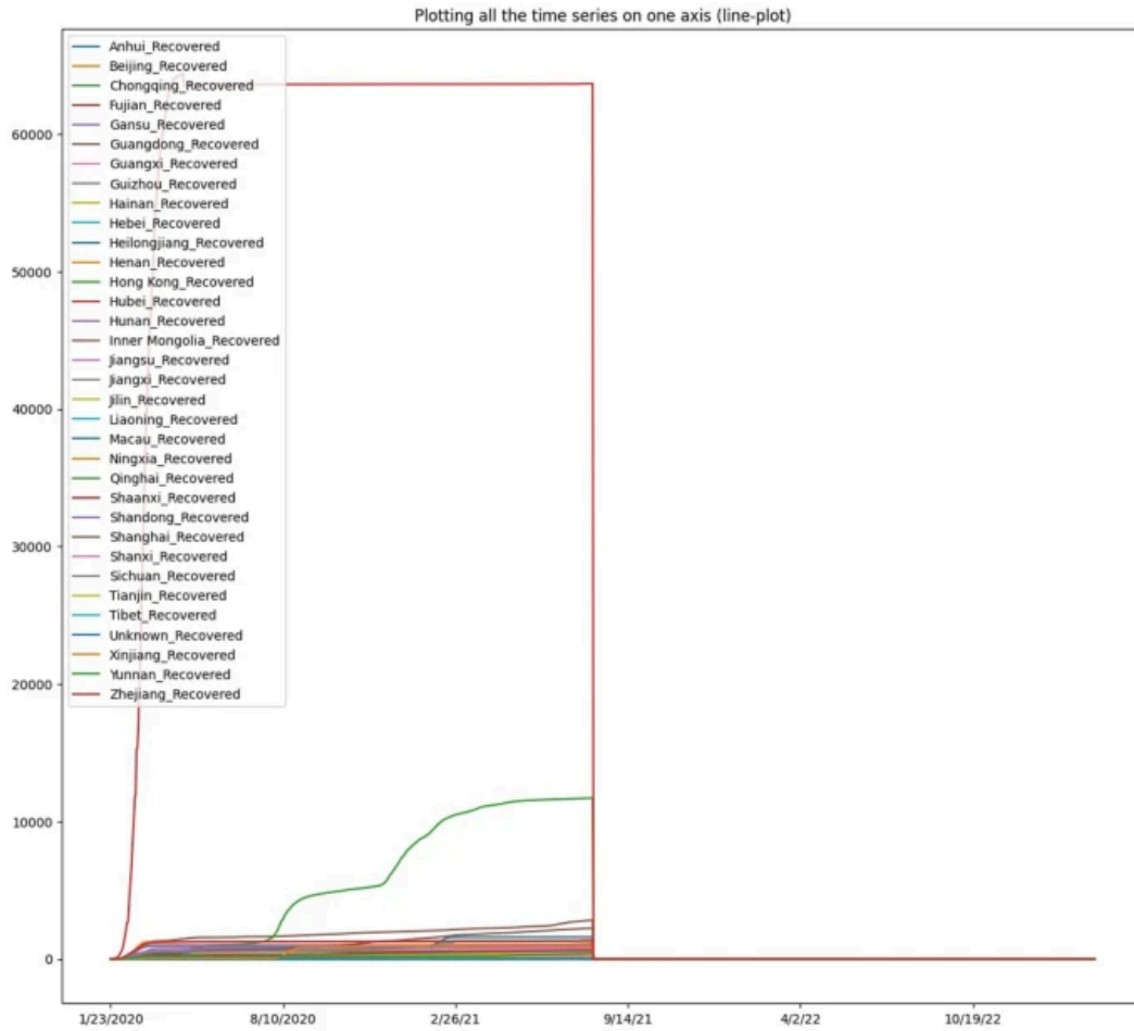
TSP of recovered cases in China
