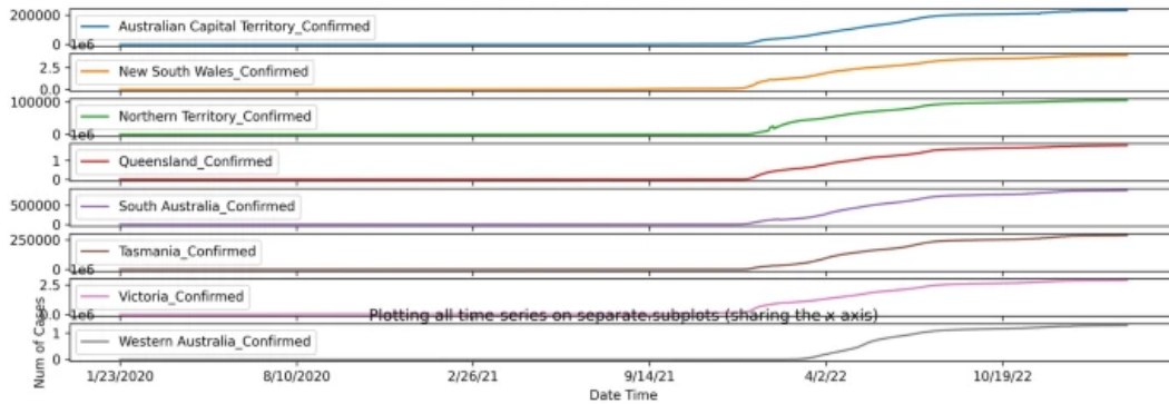
Statewide confirmed cases in Australia
