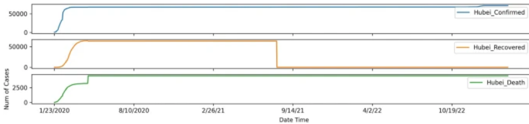
Cross-comparison of three categories in different frames
