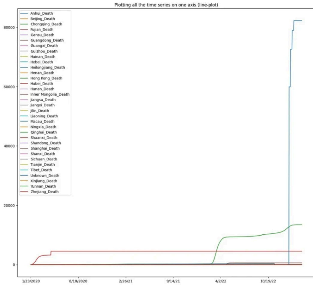
TSA of the number of death cases in China for each province
