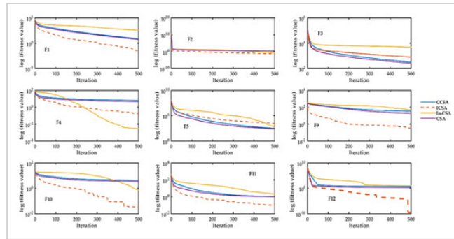
Figure 2. Convergence characteristics of conventional benchmark functions.
