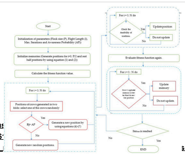
Figure 1. Flow chart of the ingenious crow search algorithm.
