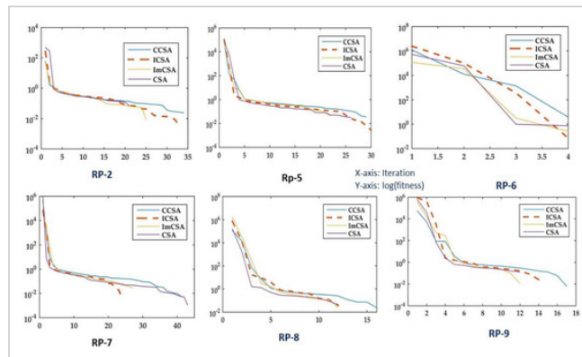
Figure 7. Convergence property analysis.
