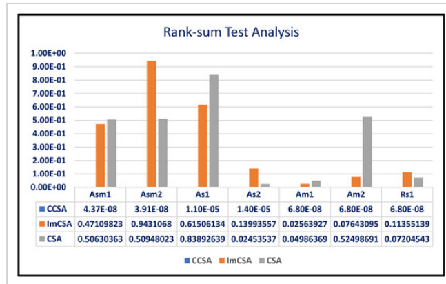
Figure 6. Rank-sum Test Analysis.
