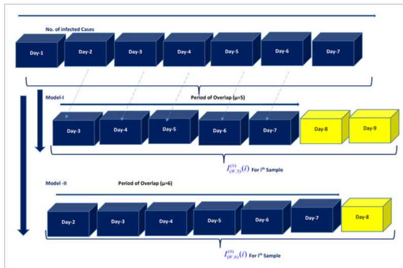
Figure 2. Proposed Rolling horizon based Grey Forecasting Models.
