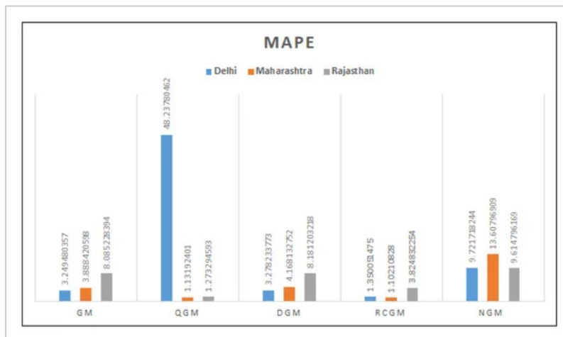
Figure 3. Forecasting Results-MAPE for Model-I.
