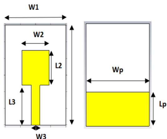
Fig.1 Front and back view of Antenna
